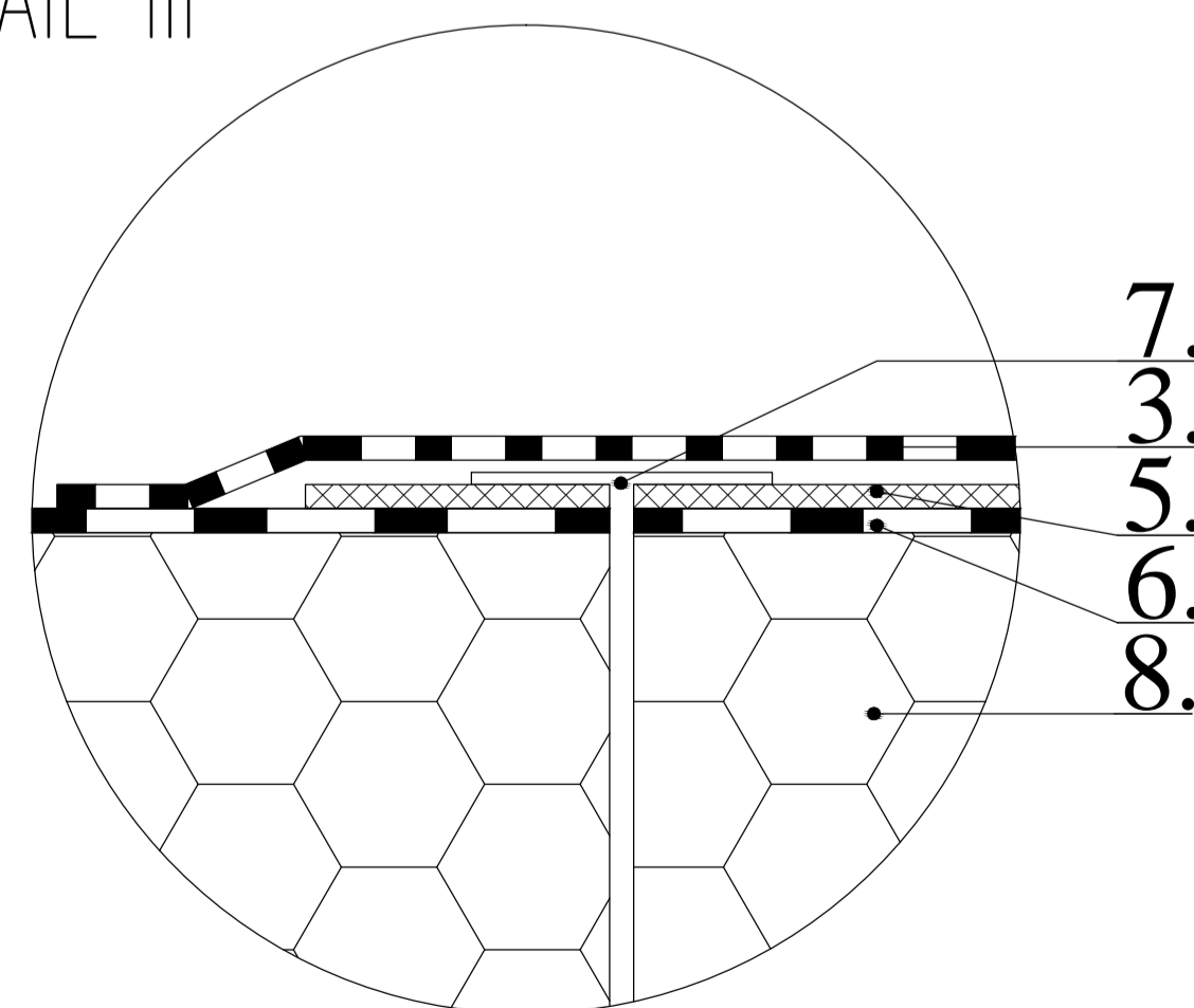
DETAIL III
